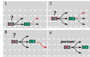
Fig. 1. We compute an action policy for the ego vehicle, in green, to disambiguate whether the red follower is in determined pursuit, or merely wandering within the bounds of standard road rules.
