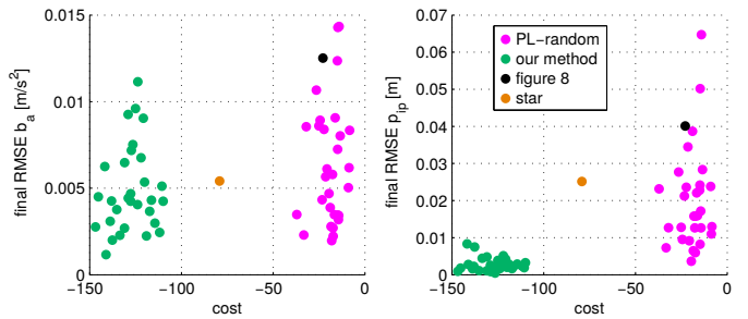
Fig. 2. Self-calibration task: final RMSE values for the accelerometer bias \mathbf{b}_a and the GPS position in the IMU frame \mathbf{p}_i^p obtained using optimization (green) and 3 different heuristics: star and figure eight trajectories from Fig. 1 and randomly sampled trajectories that are close of the physical limits of the system (magenta).
